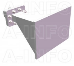
LB-159-15-C-SFSPO Standard Gain Horn Antenna 4.9-7.05GHz 15dB Gain SMA Female
