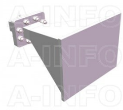
LB-159-15-C-3.5FSPO Standard Gain Horn Antenna 4.9-7.05GHz 15dB Gain 3.5mm Female
