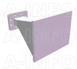
LB-159-15-ASPO Standard Gain Horn Antenna 4.9-7.05GHz 15dB Gain Rectangular Waveguide Interface
